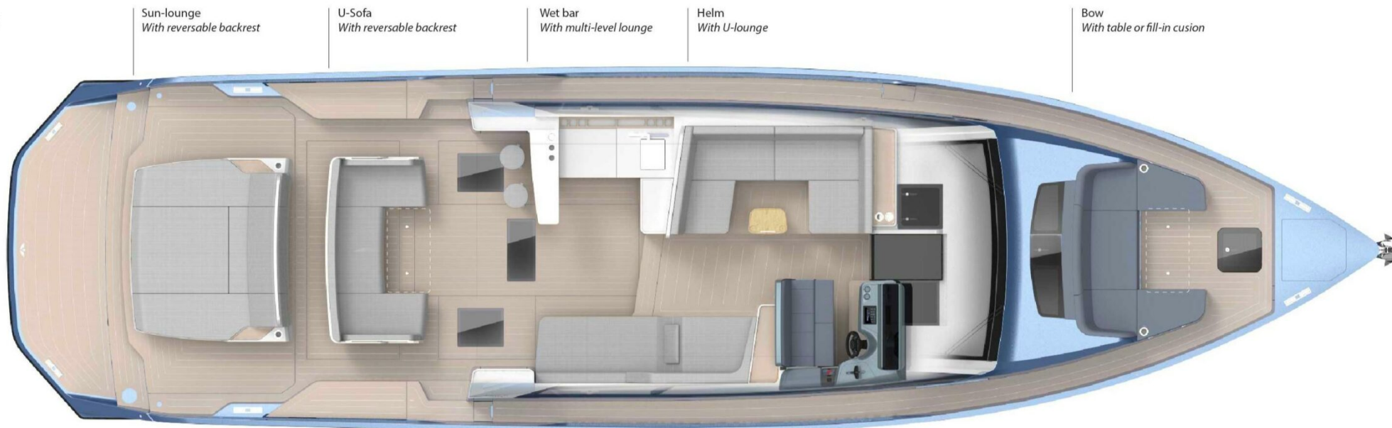
PLAN VIEW Main deck
